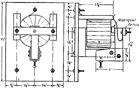
FIG. 1 POWER CONTACTOR
